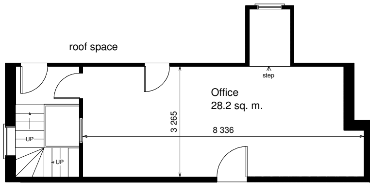
Second Floor Plan Nett usable internal floor space approx. : 28.2 sq. m.
