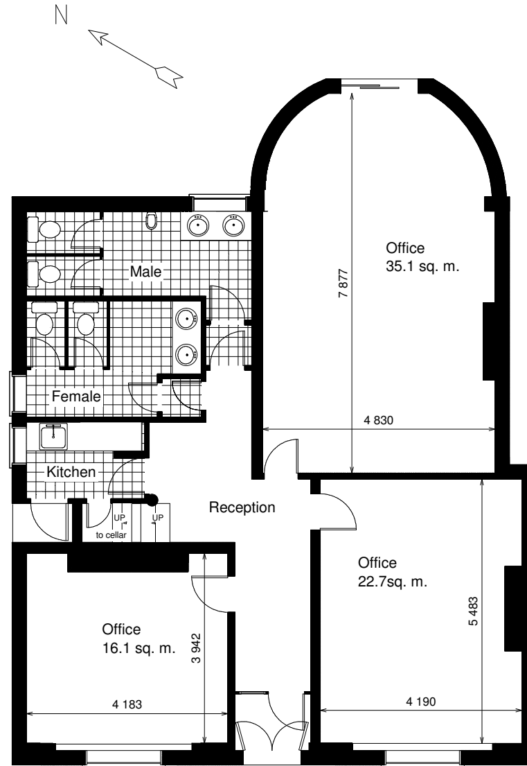
Ground Floor Plan Nett usable internal floor space approx. : 73.9 sq. m.
